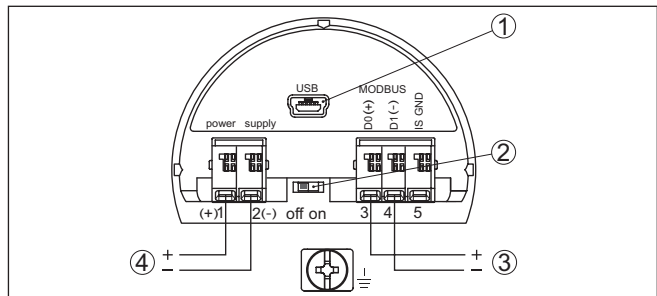
Fig. 7: Compartiment de raccordement
