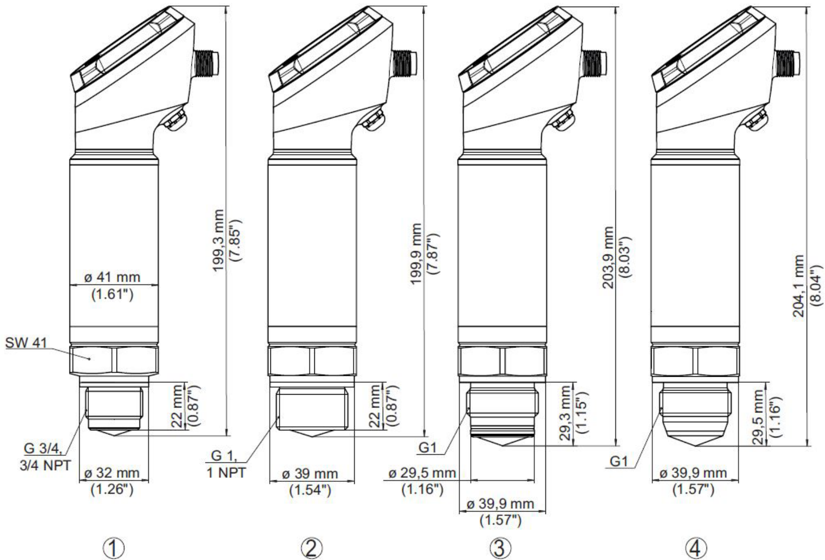
Fig. 21: Dimensions VEGAPULS 42 with display
