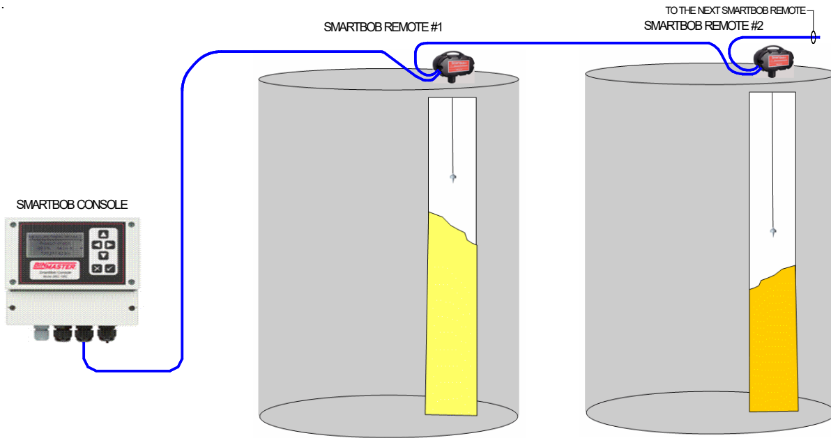
Figure 1b Console Driven SmartBob System
