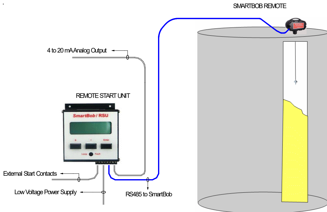
Figure 1c RSU Controlled System
