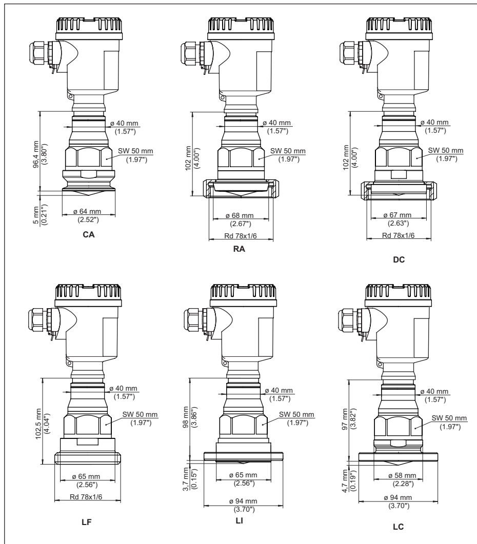
Fig. 92: NCR-86, raccord aseptique
